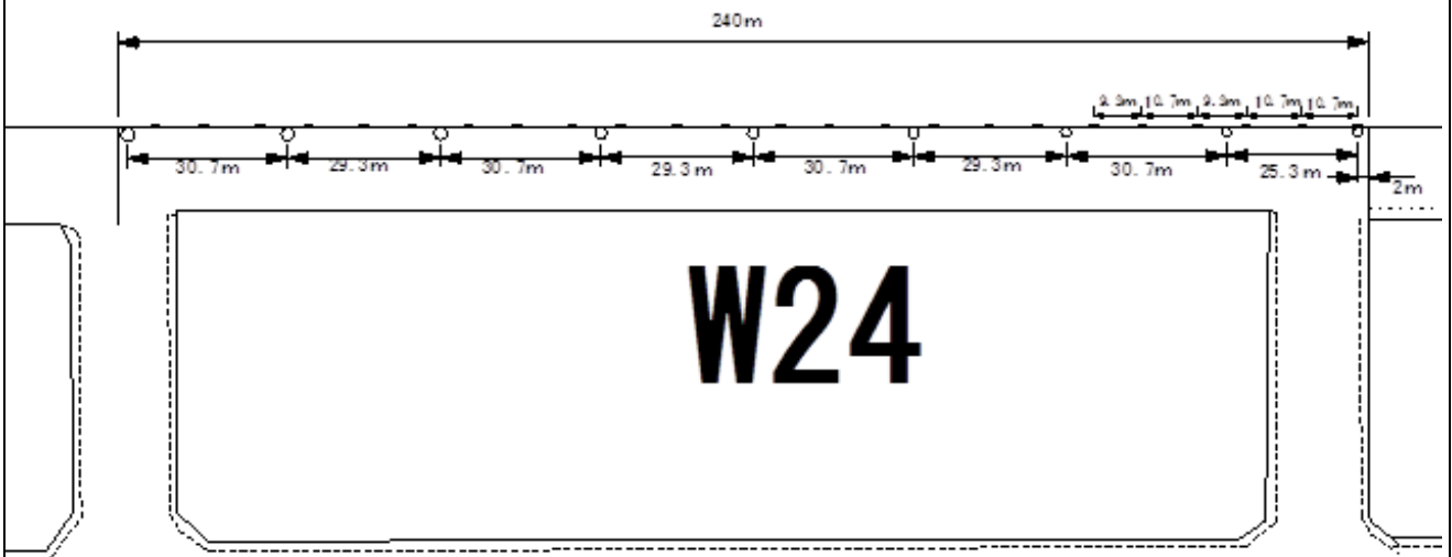
The details of a fender bar and bollard 防舷材と係船柱の詳細
